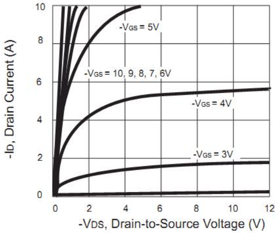
Fig 1: Output Characteristics
