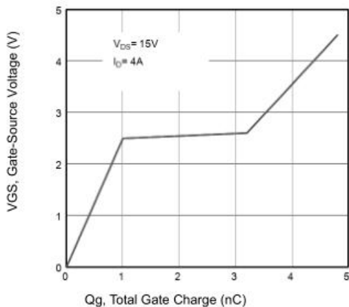
Figure 5: Gate-Charge Characteristics
