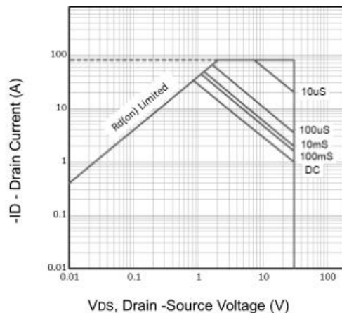
Figure 6: Safe Operating Area
