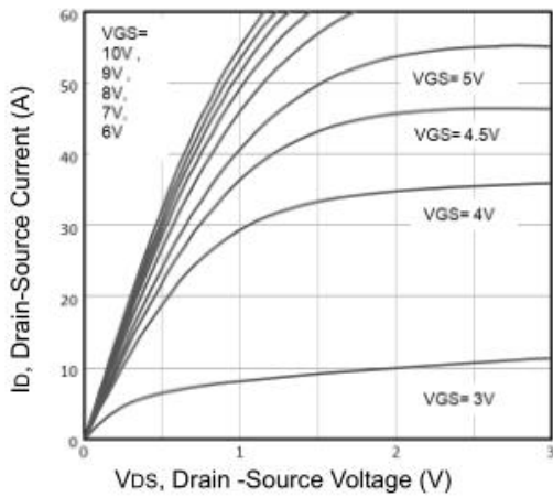
Figure 1: Output Characteristics
