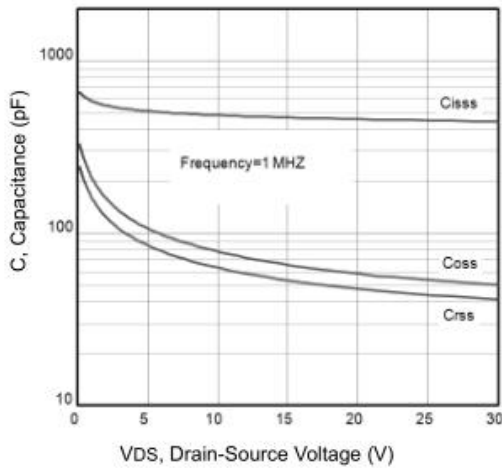
Figure 3: Capacitance
